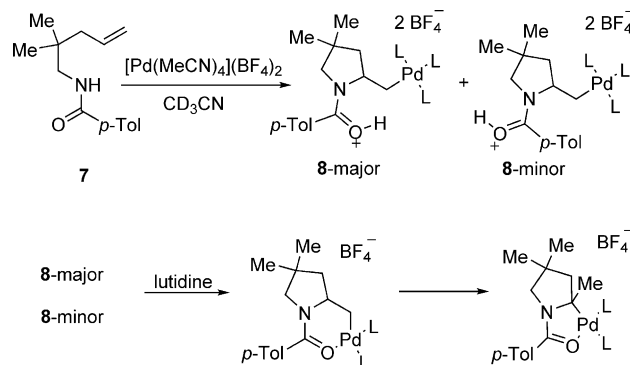
Scheme 3. Chelation-dependent rearrangement. [16]
