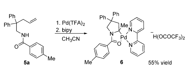
Scheme 2. Formation and isolation of palladium complex 6 .
